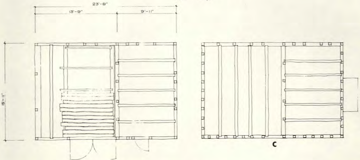
Figure 6. Steiner House Framing . a, existing framing, 1977; b, plan of existing framing; c, framing plan based on mortises in the sills and plates.
