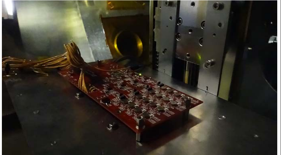
Figure 7: A photograph of the chassis-less Japanese infrasonic microphone array 'ADXII-INF02' from M.-Y. Yamamoto.
