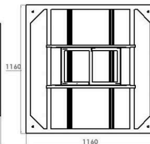
Figure 2: Top view with mounting rails
