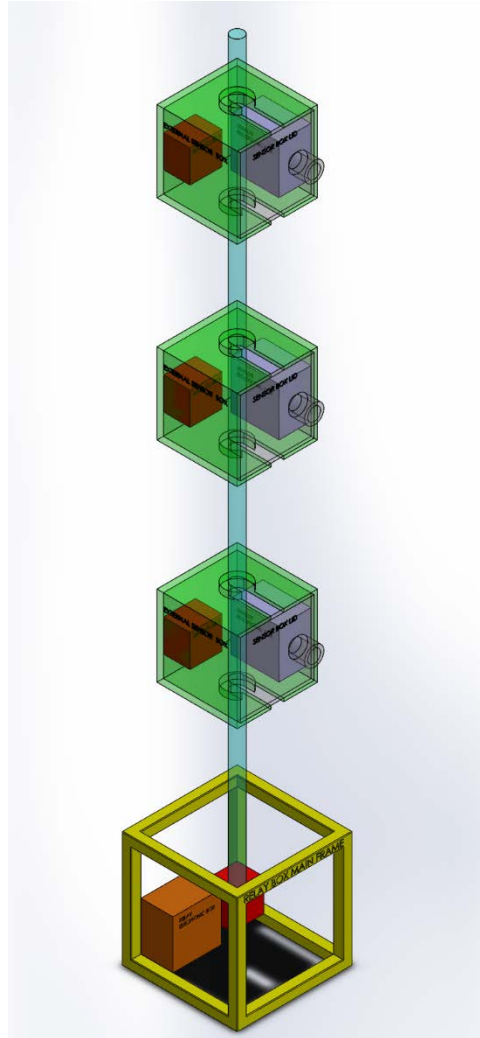
Figure 4: The set-up on the gondola and flight train. The green boxes are the sensor boxes, while the devices inside the yellow frame are the relay box devices within the gondola space. This model is not to scale.
