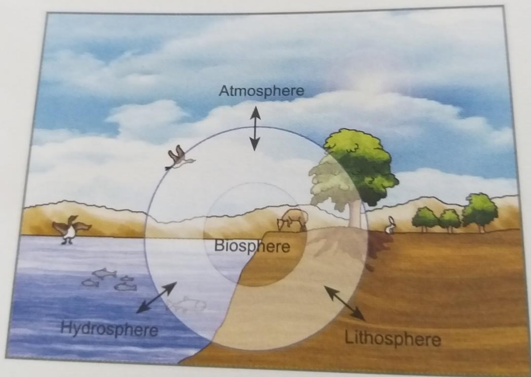
Fig. 1.1: The four domains of the Earth
