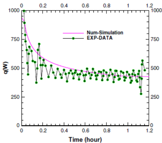
Fig. 4. Heat rate transferred to the storage tank versus time for \dot{m}_{in} = 75\% , T_{air\ in} = 24\ ^\circ\text{C} and \dot{m} = 0.0766\ \text{Kg s}^{-1} .
