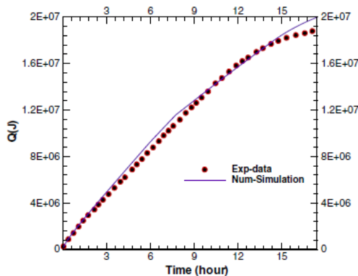
Fig. 5. Total of heat rate transferred to the storage tank versus time for \dot{m}_{in} = 75\% , T_{air\ in} = 24\ ^\circ\text{C} and \dot{m} = 0.0766\ \text{Kg s}^{-1} .
