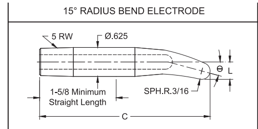
15° RADIUS BEND ELECTRODE
