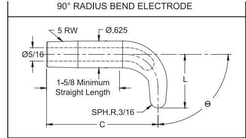
90° RADIUS BEND ELECTRODE
