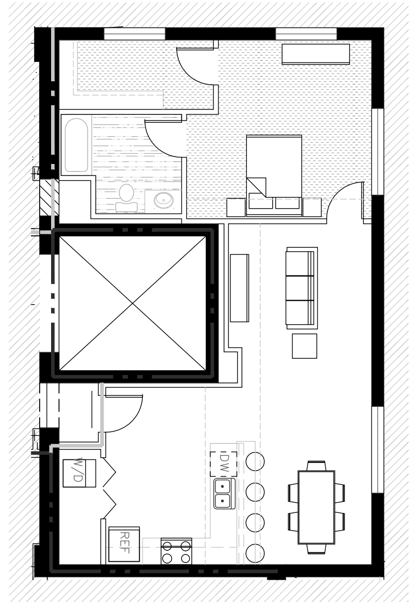
FLOOR PLAN F 1 BR / 1 BATH
