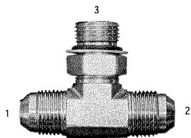
Male JIC X Male ORB Tee
