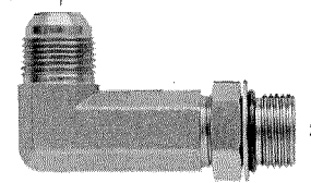
Male JIC x Male ORB 90° Bend "X-Long"
