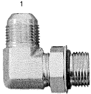
Male JIC x Male ORB 90° Bend
