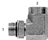
Male ORB x Female Rigid NPT 90° Bend
