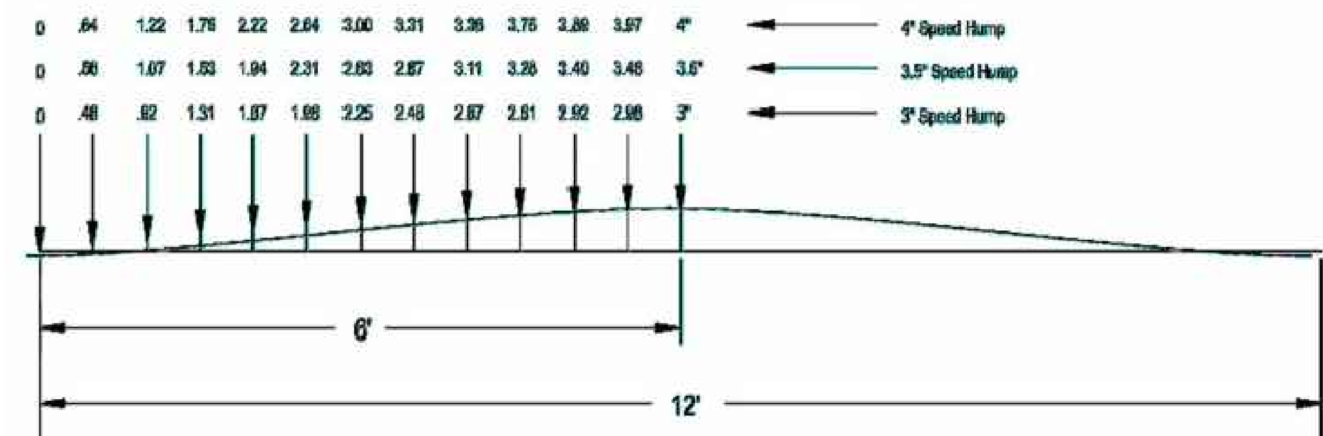
SPEED HUMP CROSS-SECTION DETAIL
