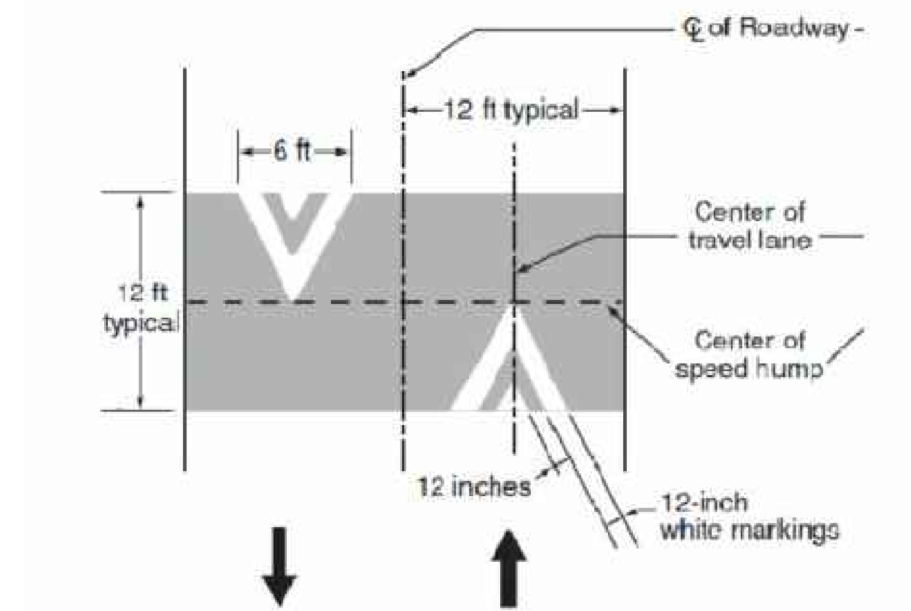
SPEED HUMP PAVEMENT MARKING DETAIL
