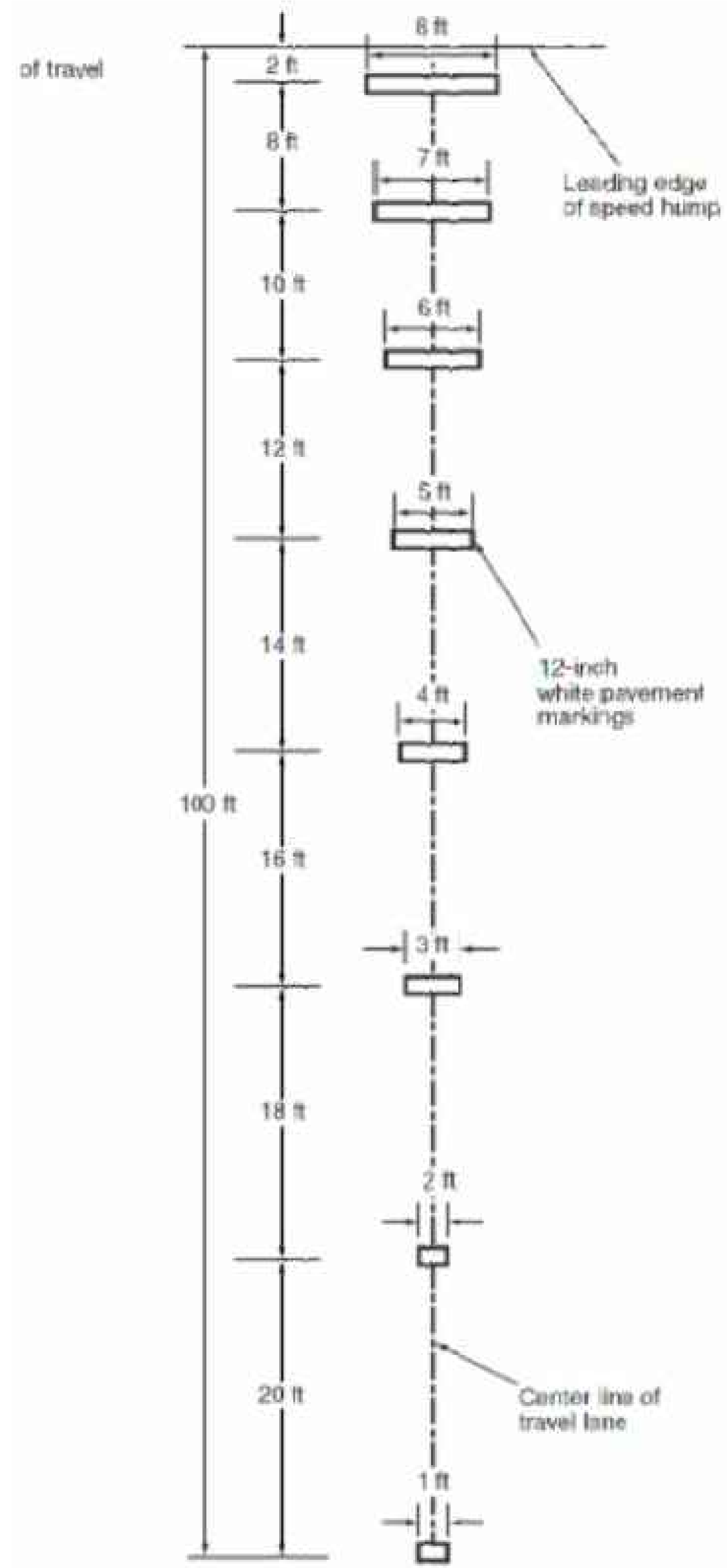
SPEED HUMP ADVANCE WARNING MARKING DETAIL
