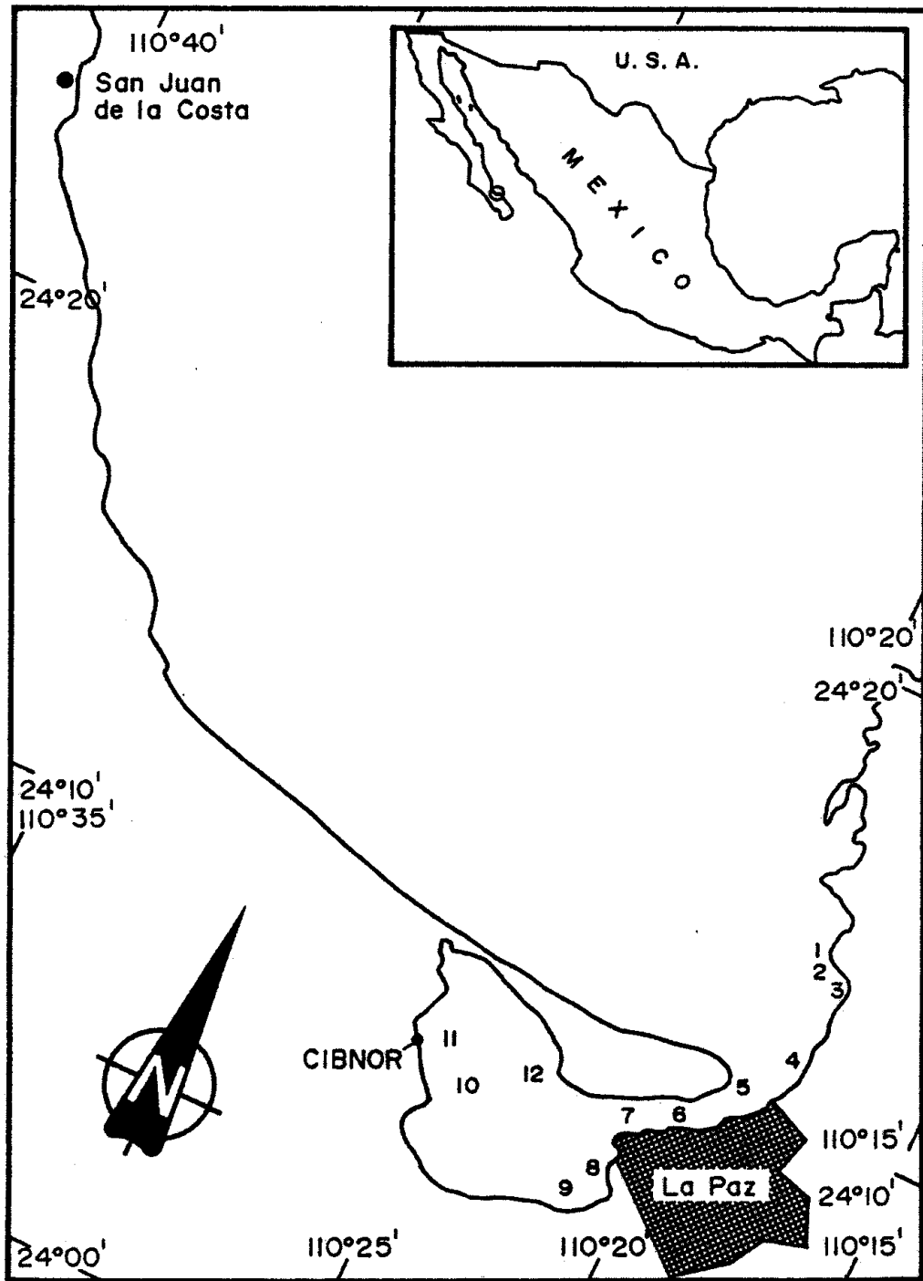
Figure 1. Location of the stations in Bahía and Ensenada de La Paz, México
