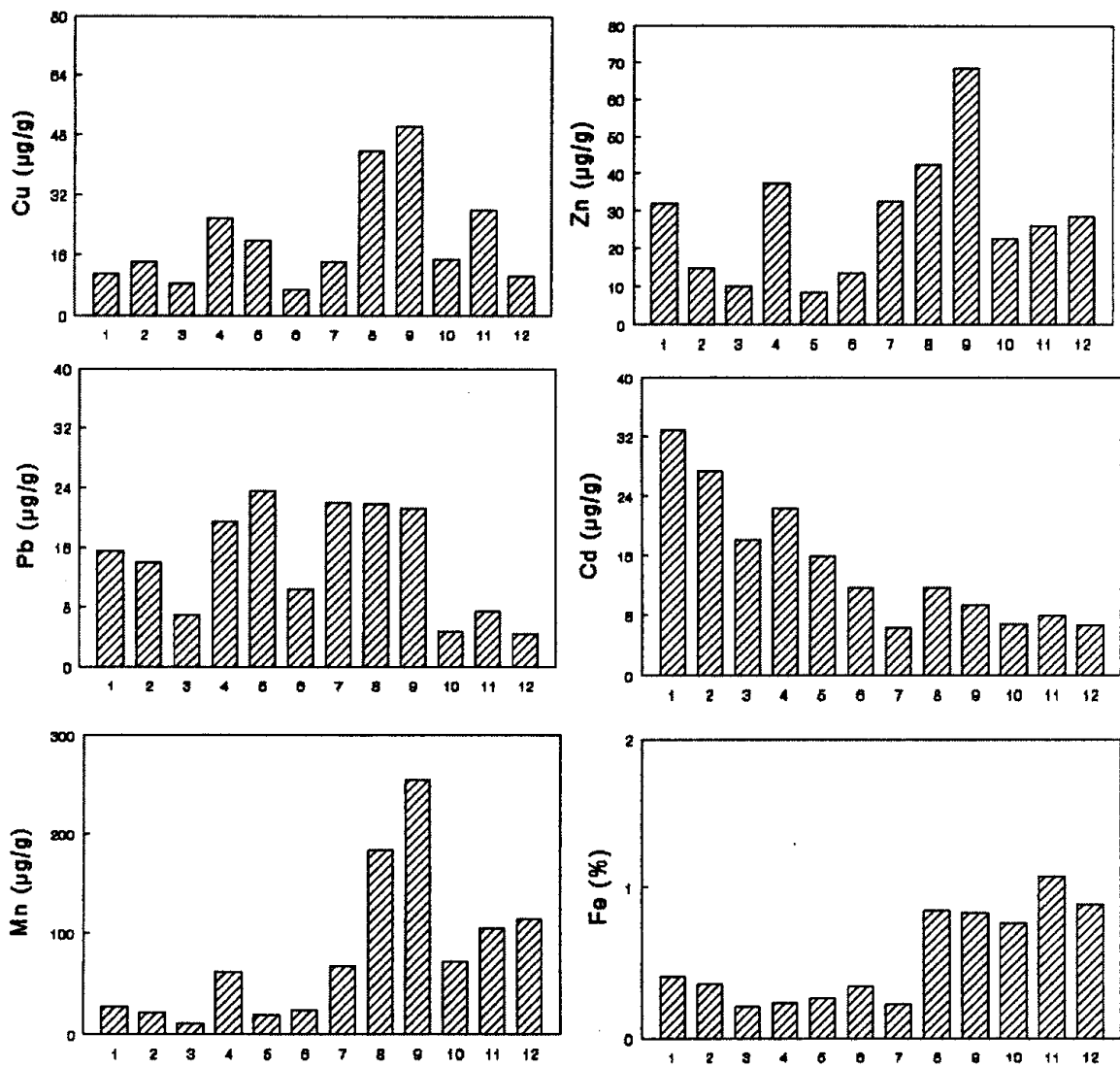
Figure 2. Metal levels at twelve stations from Bahía and Ensenada de La Paz, México.
