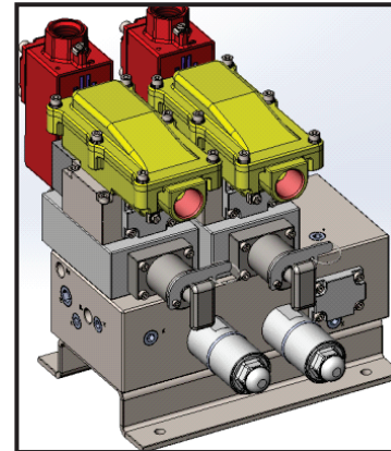
2oo2 VOTING SYSTEM DOUBLE MODULAR REDUNDANCY
