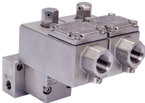
2oo2 Voting System - in Manifold .
