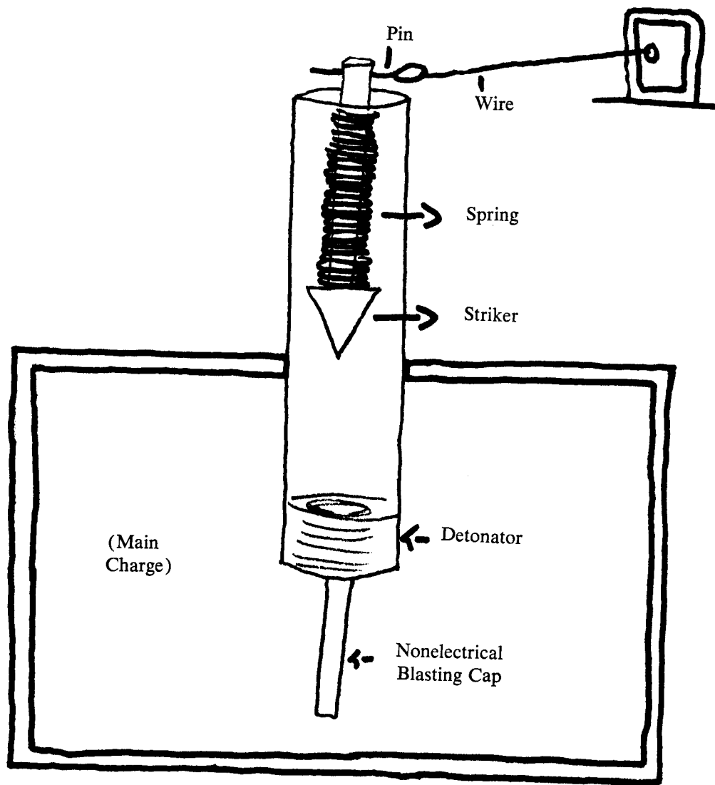
Figure 89. Tension-release detonator.
