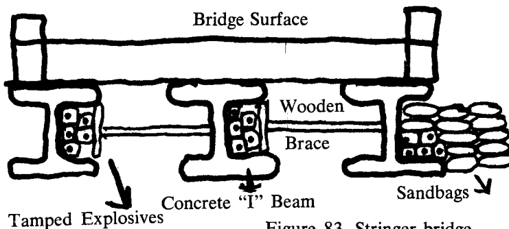
Figure 83. Stringer bridge.
