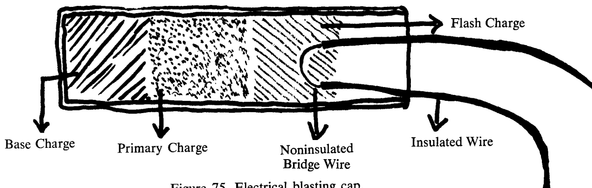
Figure 75. Electrical blasting cap.
