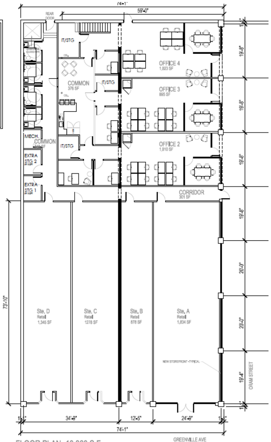
FLOOR PLAN -10,360 S.F. 2000 GREENVILLE AVE
