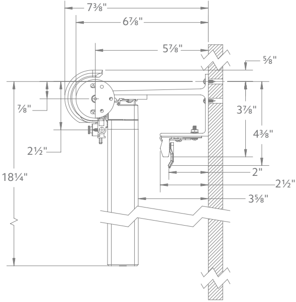
2" DOUBLE MOUNT WITH SUPERFINE™
