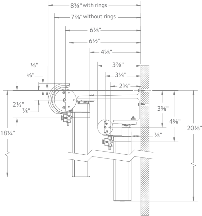
2" & 1 3/8" DOUBLE STAGGERED MOUNT
