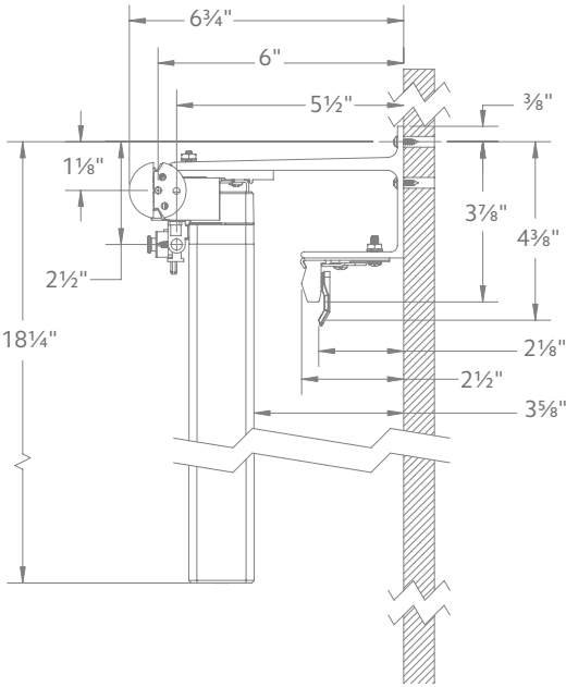
1 3/8" DOUBLE MOUNT WITH SUPERFINE™
