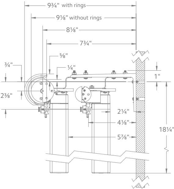
2" & 1 3/8" DOUBLE MOUNT
