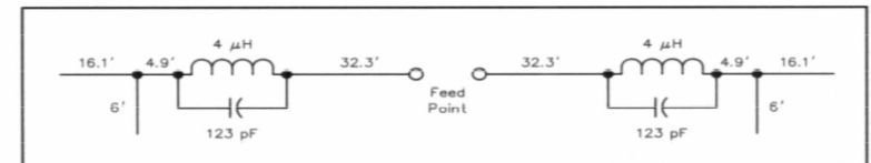
Figure 1—A W8NX multiband dipole for 80, 40, 20, 15 and 10 meters. The values shown (123 pF and 4 μH) for the coaxial-cable traps are for parallel resonance at 7.15 MHz. The low-impedance output of each trap is used for this antenna.
