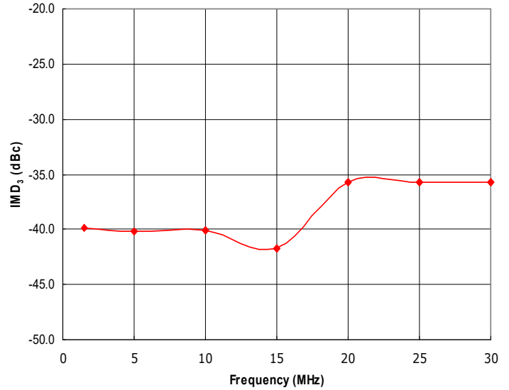
Figure 2: RFP1.5-30-100XR Typical IMD 3 @ 100W PEP, Δf=10kHz. For unbalanced IMD 3U and IMD 3L , only the highest value is shown.
