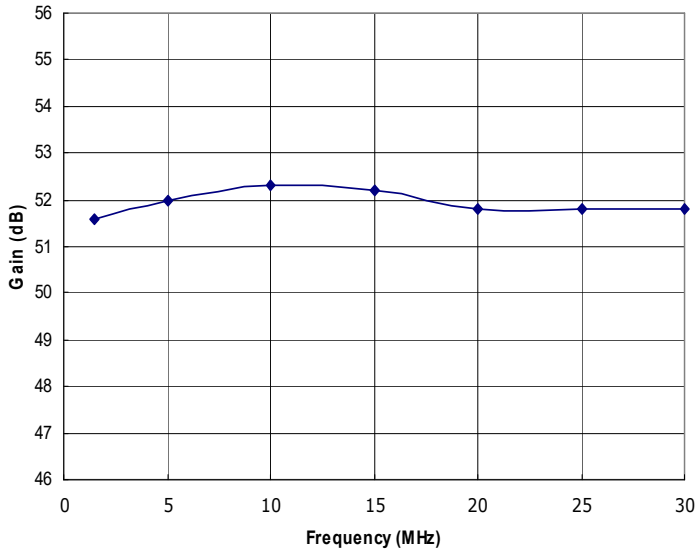
Figure 1: RFP1.5-30-100XR Typical Gain @ P out = 100W.
