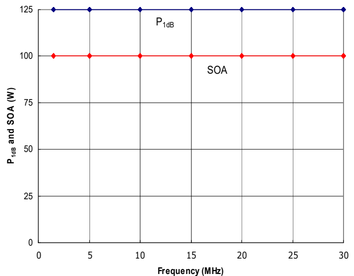
Figure 4: RFP1.5-30-100XR Typical P 1dB and Safe Operating Area (SOA). Do not exceed the SOA without first contacting RFMPT to discuss your application.
