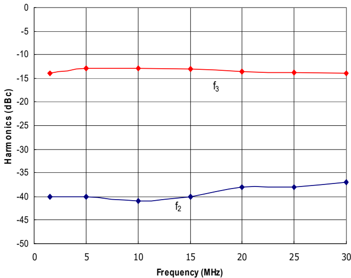
Figure 3: RFP1.5-30-100XR Typical f 2 and f 3 @ P out = 100W.
