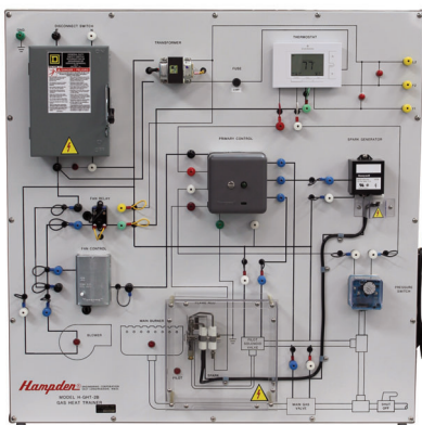
Model H-GHT-2B Gas Heat Trainer Dimensions: 36"H x 36"W x 13"D Shipping Wt.: 260 lbs.
