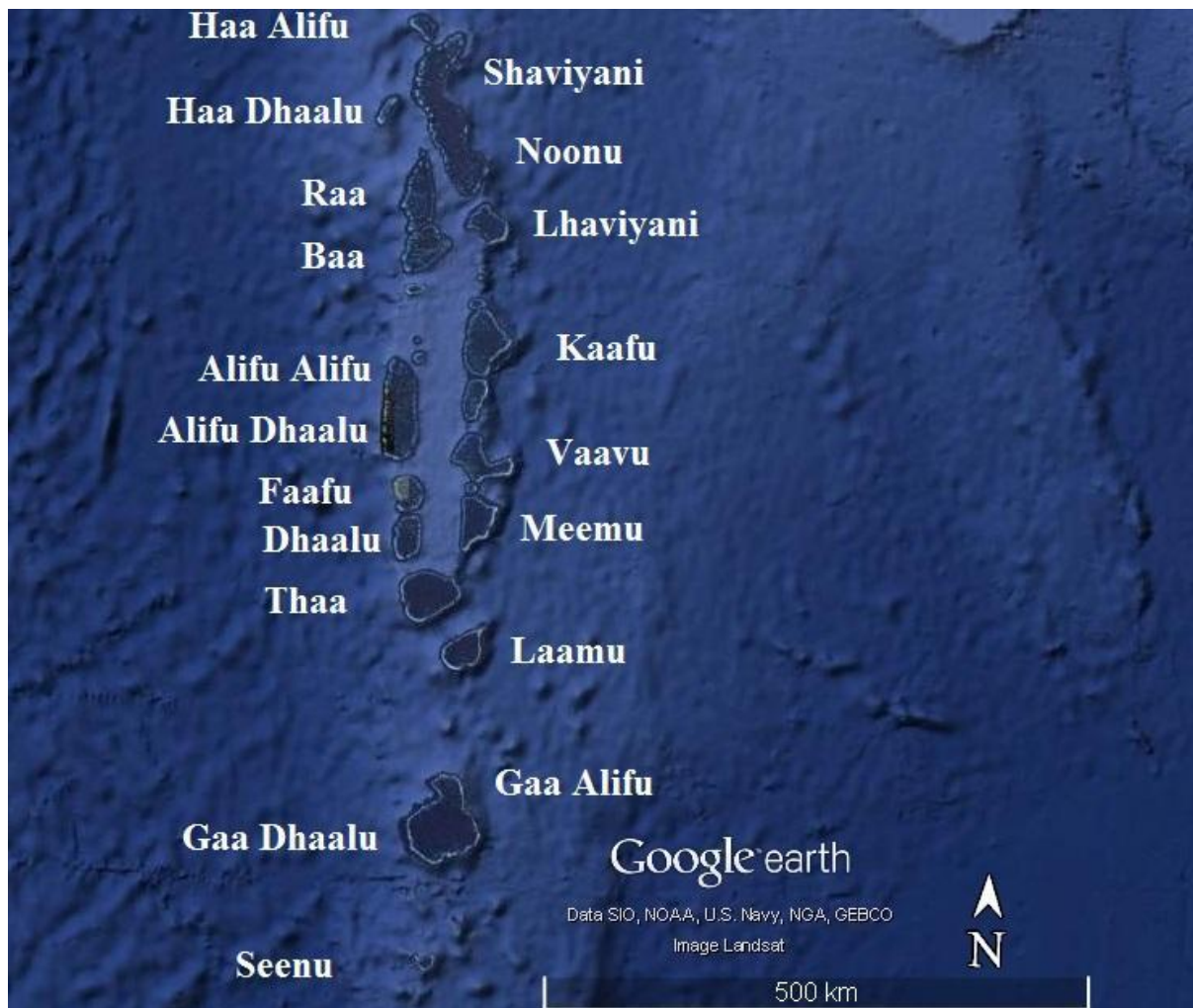
Fig. 2. The atolls of the Maldives
