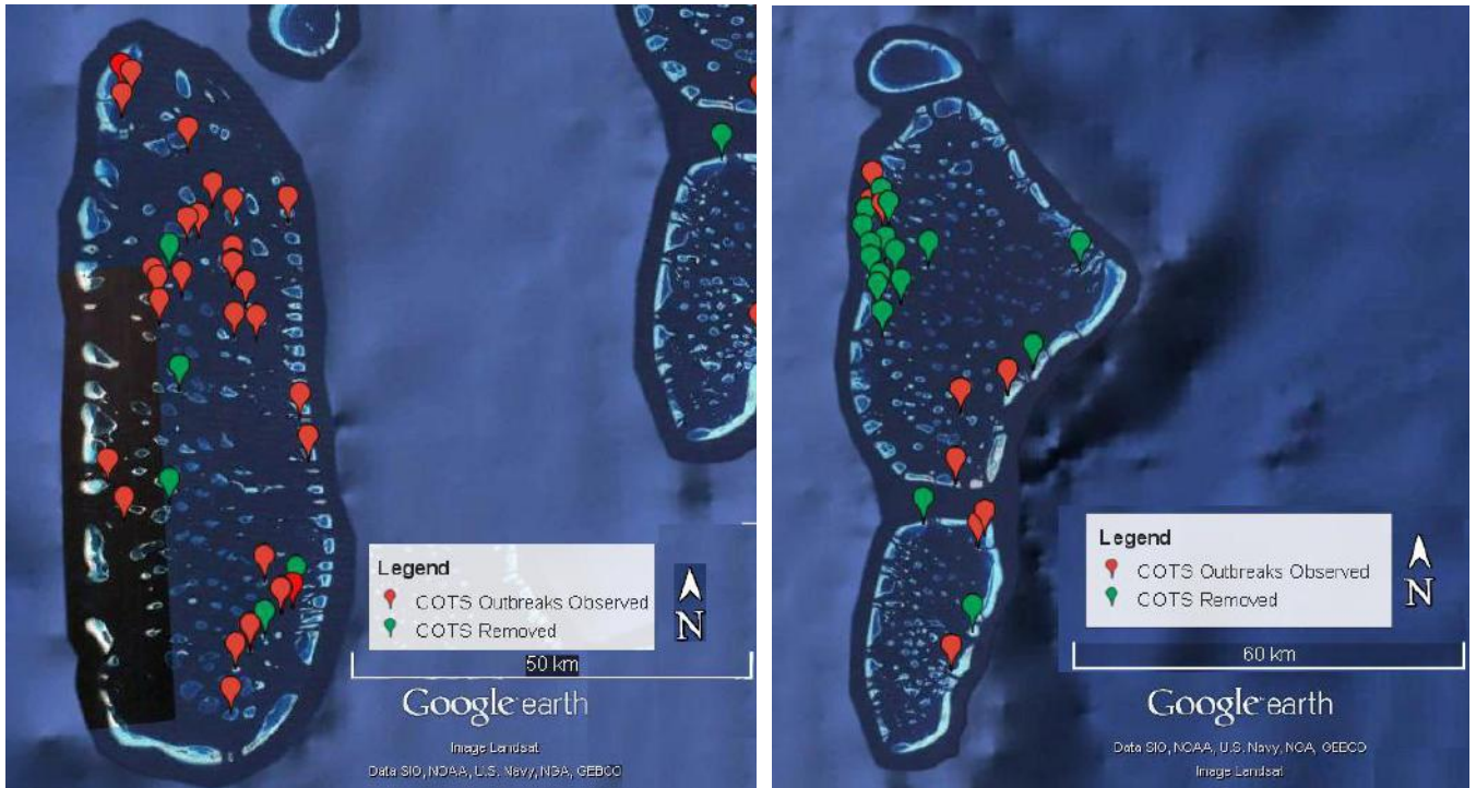
Fig. 34. Location of COTS outbreaks and COTS removals on Ari Atoll (left) and North and South Malé Atoll.
