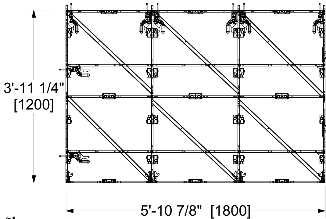
Front View 3/4" = 1'0"
