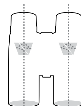
ROOF PRISM
