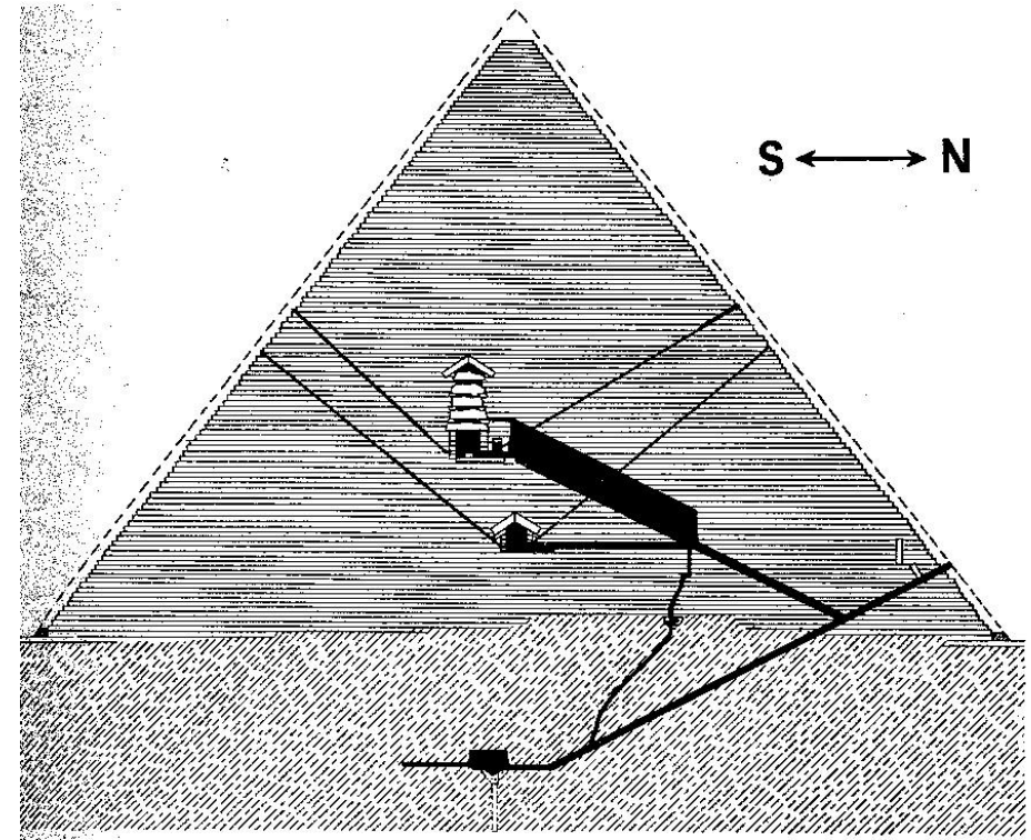
This graphic is a layout of the chambers and passages of the great pyramid 1
