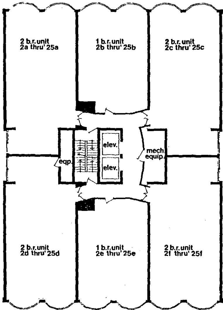
Plan of Floors 2 thru' 25
