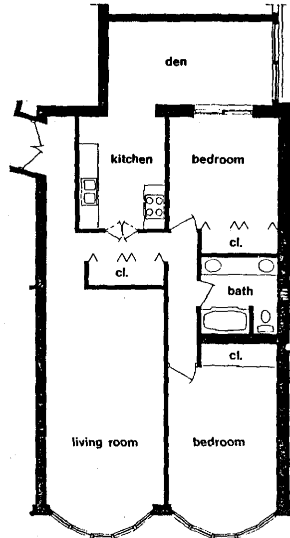
2 Bedroom Unit Floors 2 thru' 25
