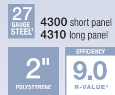
2" 1 3/8" Polystyrene Models
