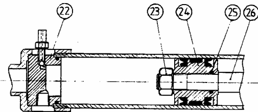
UNBALANCED CYLINDER
