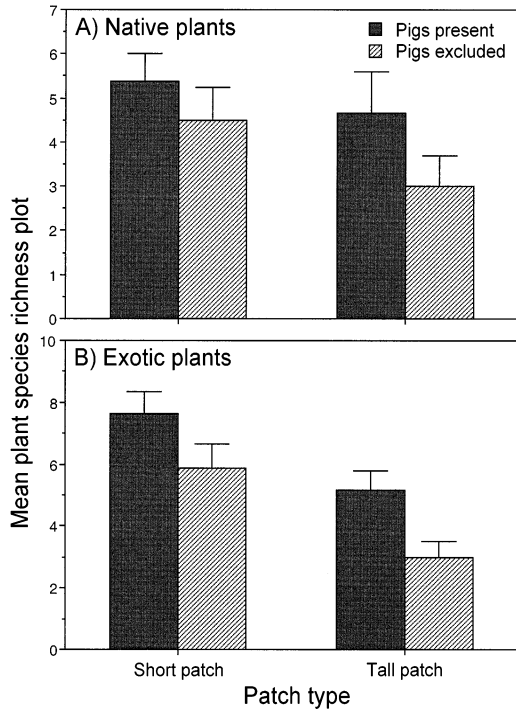
FIG. 2. Plant species richness (mean + 1 SE) of (A) native and (B) exotic taxa as a function of short and tall patch types and whether feral pigs and their soil disturbances were present or excluded.
