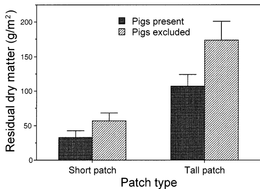
FIG. 4. Residual dry matter (mean + 1 SE) as a function of short and tall patch types and whether feral pigs and their soil disturbances were present or excluded.
