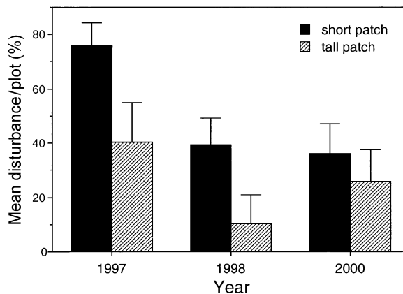
FIG. 1. Percentage area of plots (mean + 1 SE) that were disturbed by feral pigs in each of three years (1997, 1998, and 2000) in short and tall patch types.
