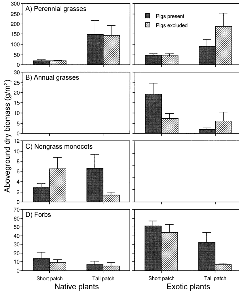
FIG. 3. Aboveground dry biomass (mean + 1 SE) of native and exotic plants as a function of short and tall patch types and whether feral pigs and their soil disturbances were present or excluded. Plants were grouped into functional groups: (A) perennial grasses, (B) annual grasses, (C) nongrass monocots (primarily bulbs), and (D) forbs.
