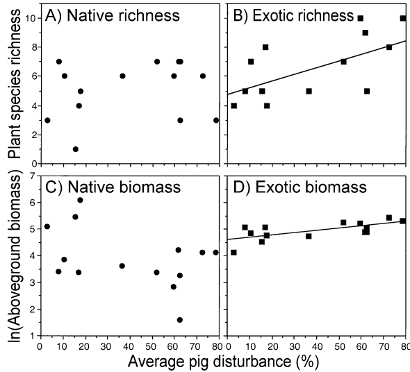
FIG. 5. Relationship between (A, B) plant species richness and (C, D) aboveground dry biomass (g/m 2 ) and percentage pig disturbance averaged over three years (1997, 1998, and 2000) for both native and exotic taxa.
