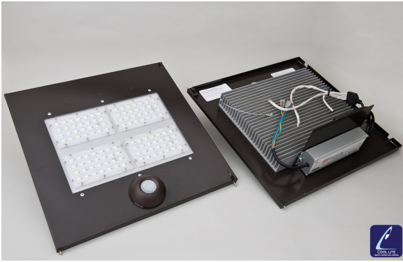
Gardco Form 10 Shoebox Retrofit Kit
