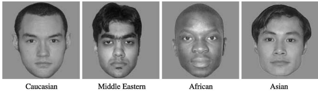
Figure 1. Sample stimuli.
