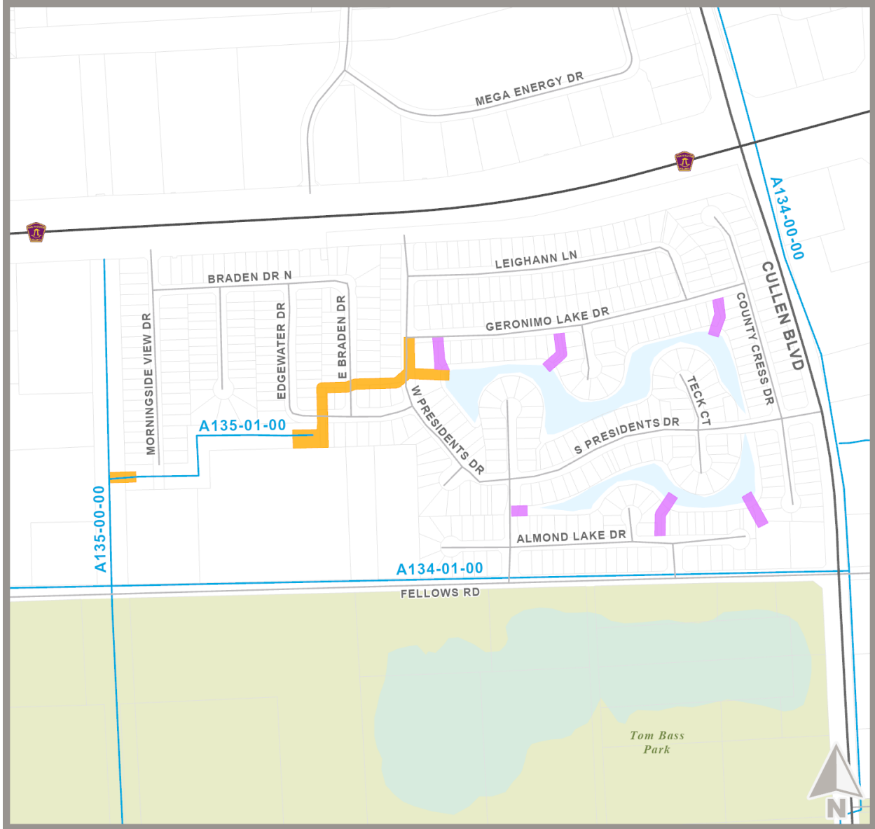
A135-01-00-E001 Channel Conveyance Improvements
