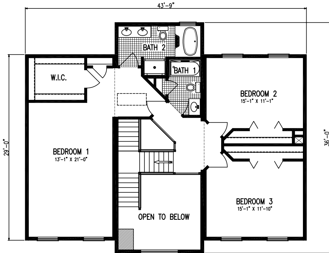
2ND FLOOR- 1367 SQ FT
