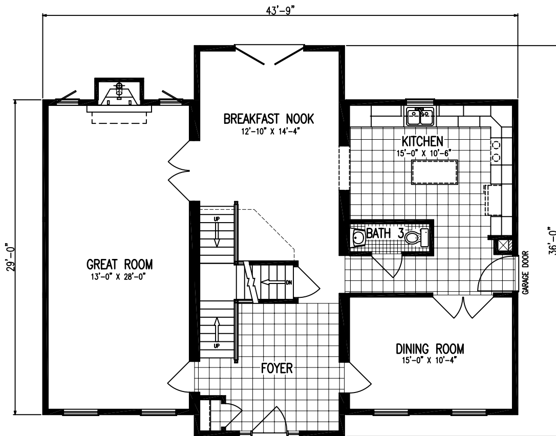
1ST FLOOR- 1367 SQ FT
