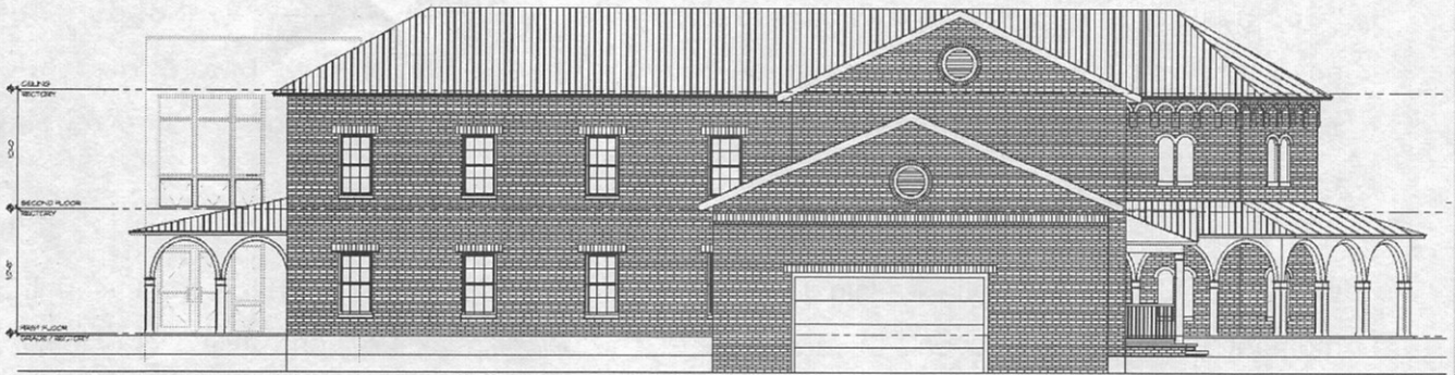
West Elevation – View from School Lane
