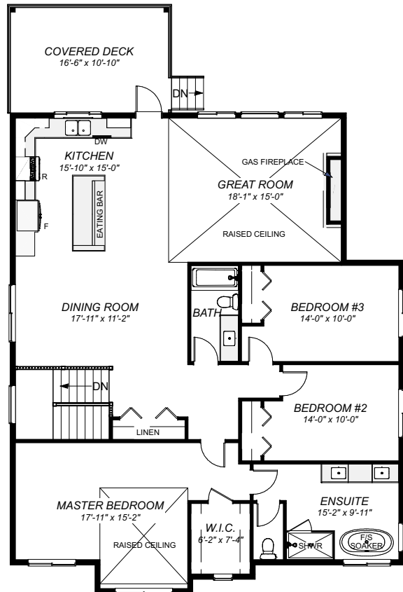
MAIN FLOOR PLAN 1800 sq ft
