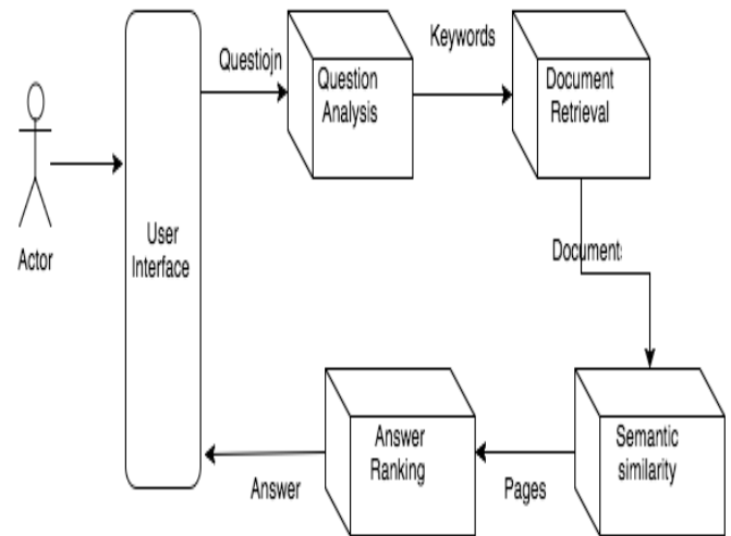
Figure 1. Block Diagram Question Answering System
