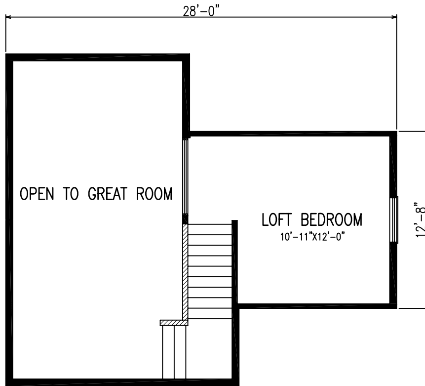
OPTIONAL 2ND FLOOR-170 SQ FT
