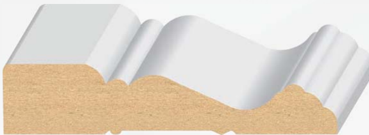
155MUL 11/16 x 3-1/2 Ultralight Cape Cod Casing N/S
