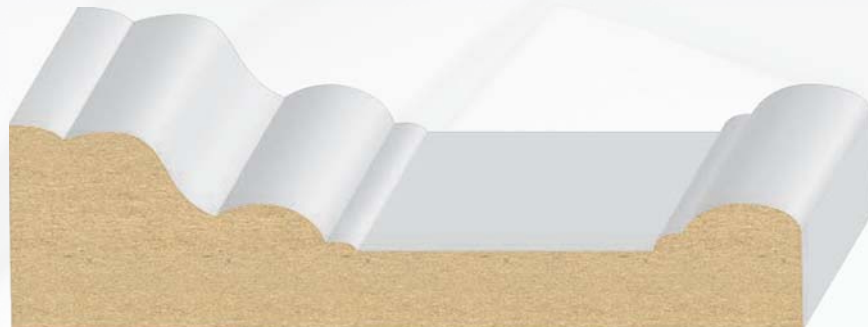
174MUL 1-1/8 x 4-1/8 Ultralight Howe Casing N/S
