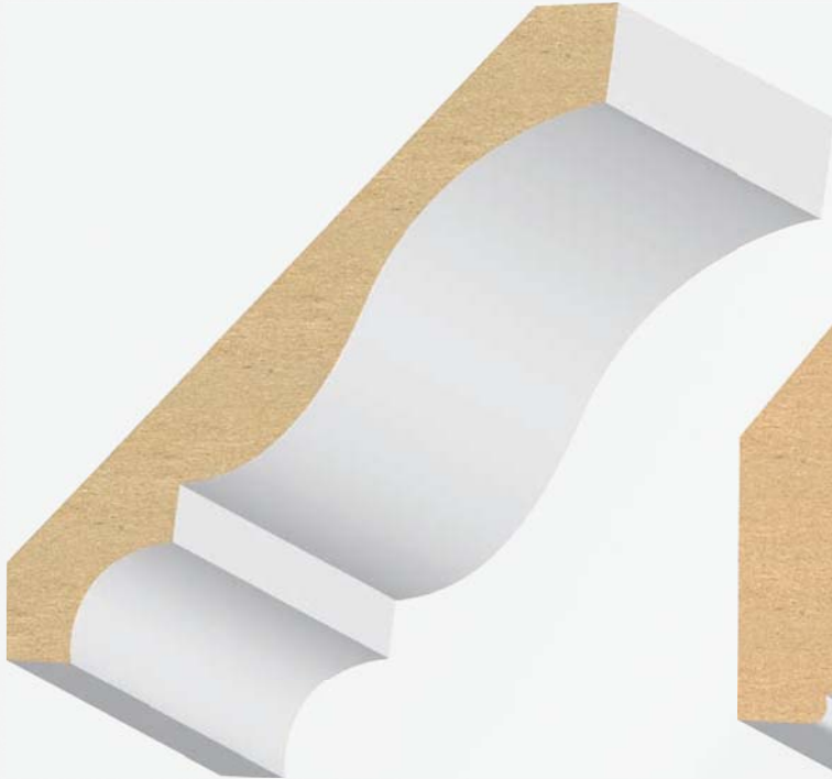
446MUL 5/8 x 3-5/8 Ultralight Colonial Crown N/S
