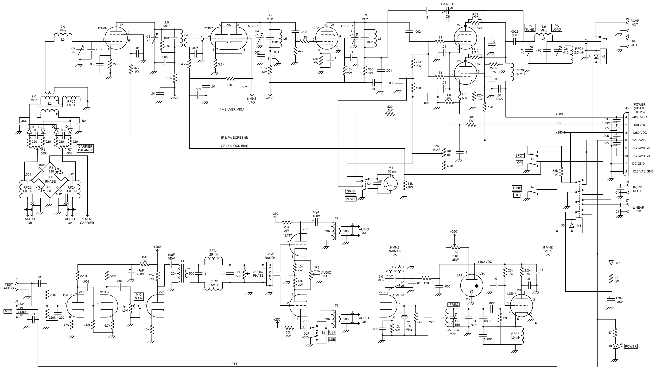
80 METER CHEAP 'N EASY II HOMEBREWED BY KG7TR MAY, 2013
