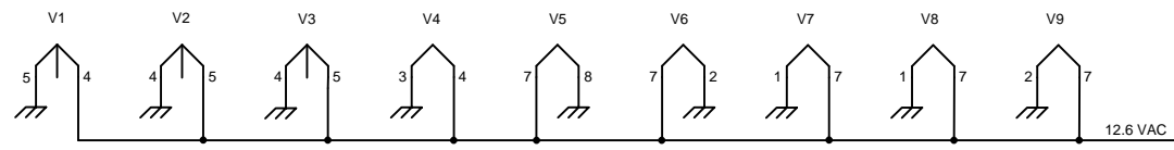
80 METER CHEAP 'N EASY II HOMEBREWED BY KG7TR MAY, 2013
