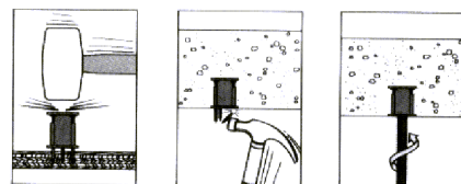
Wood Form Insert Installation Sequence
