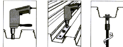
Metal Roof Deck Insert Installation Sequence
