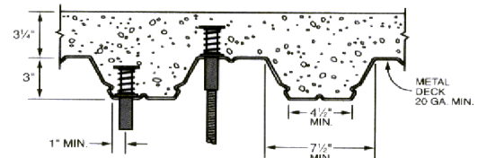
Typical Metal Deck Installation
