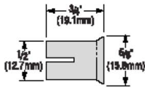
Short Drop-In Dimensions
