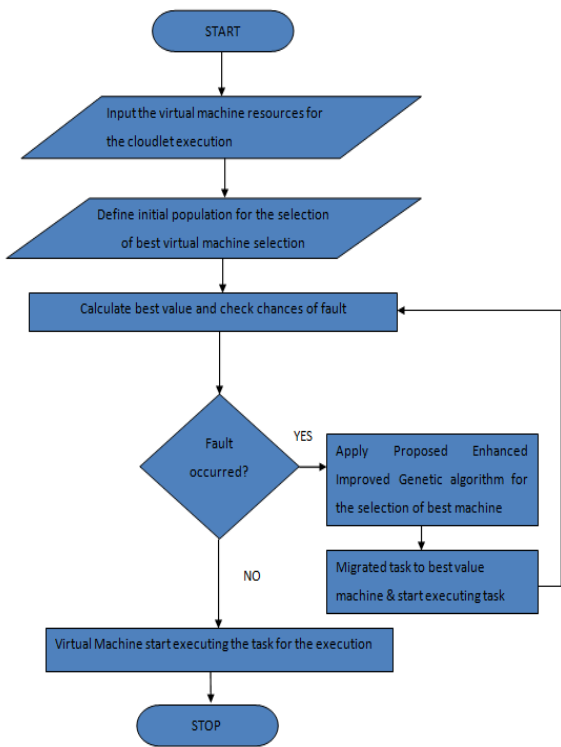
Figure 1: Flowchart of Proposed Enhanced Improved Genetic Algorithm
