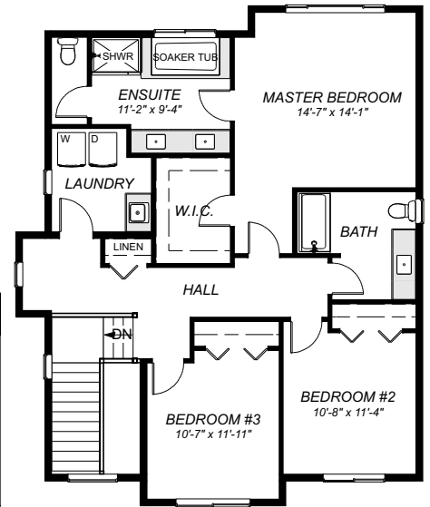
UPPER FLOOR PLAN 1164 sq ft
