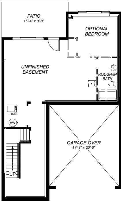
LOWER FLOOR PLAN 897 sq ft
