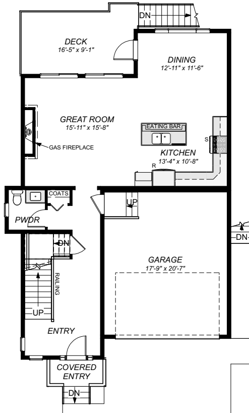
MAIN FLOOR PLAN 913 sq ft
