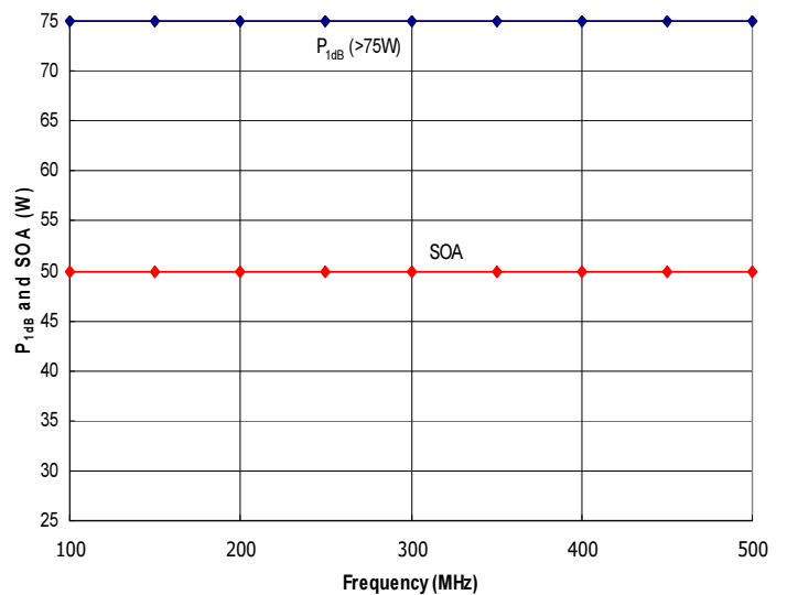
Figure 4: RFM100-500-50-HSD Typical P 1dB and Safe Operating Area (SOA). The amplifier is capable of delivering much more power than it is safe to generate. Do not exceed the SOA shown above without first contacting RFMPT to discuss your application.
