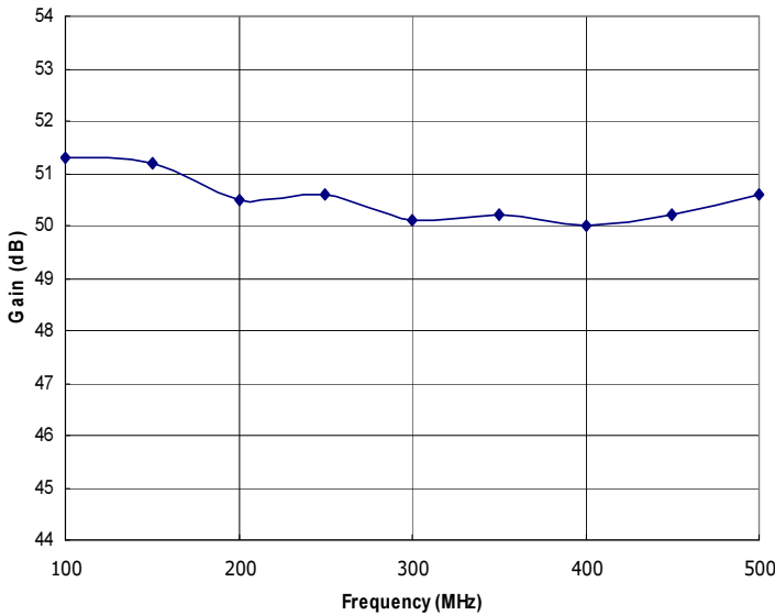
Figure 1: RFM100-500-50-HSD Typical Gain @ P out =50W.
