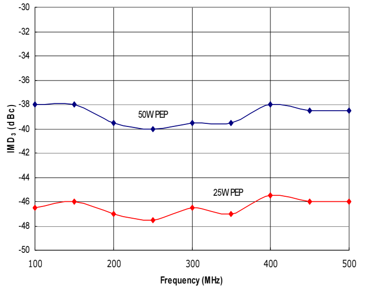
Figure 2: RFM100-500-50-HSD Typical IMD 3 @ 50W and 25W PEP, Δf=10kHz and Δf=100kHz.
