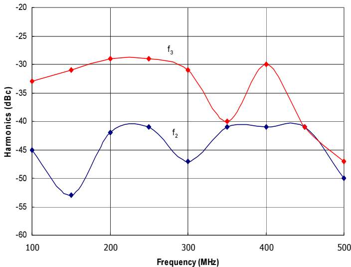
Figure 3: RFM100-500-50-HSD Typical f 2 and f 3 @ P out =50W.
