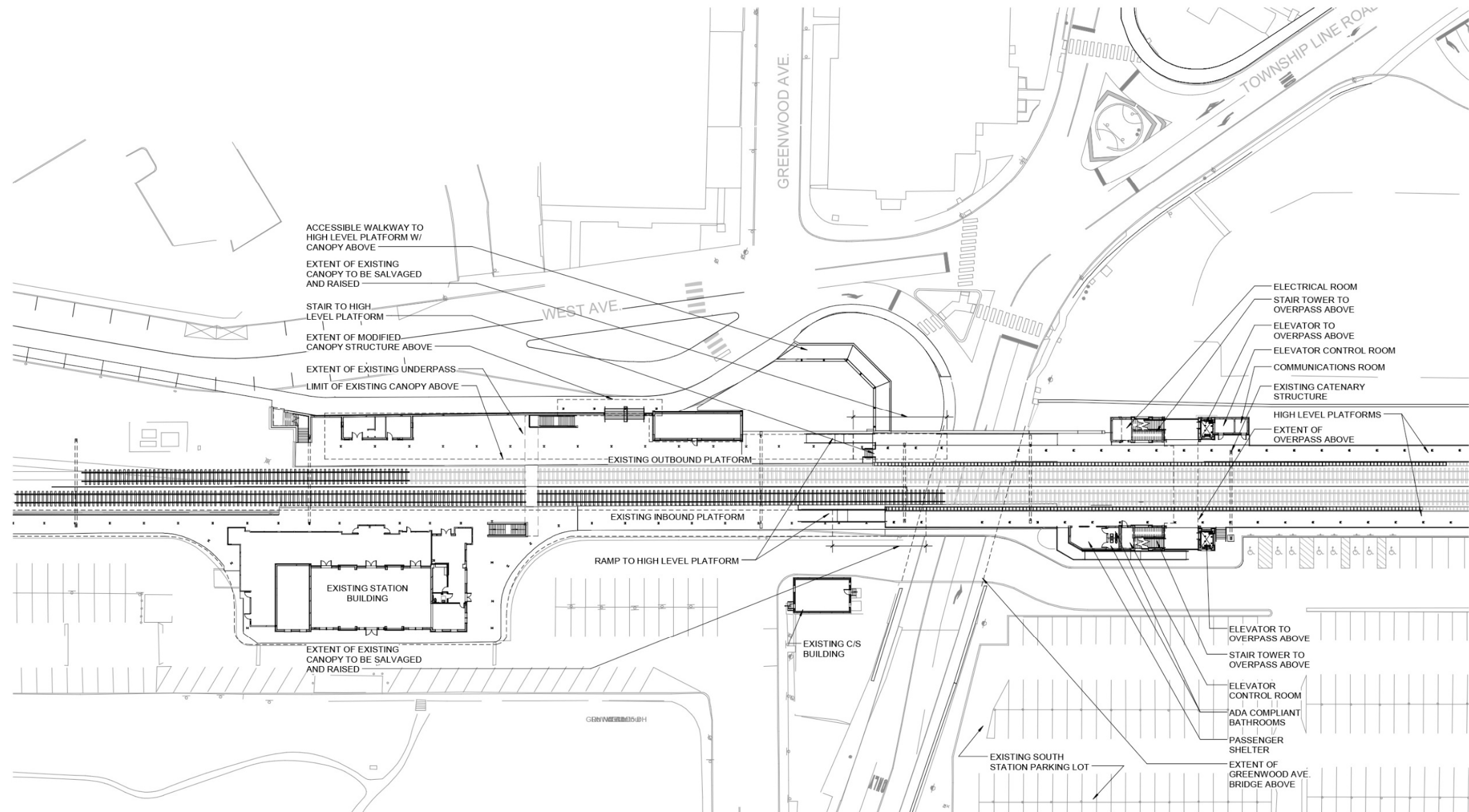
Figure B3 Enlarged Proposed Station Plan
