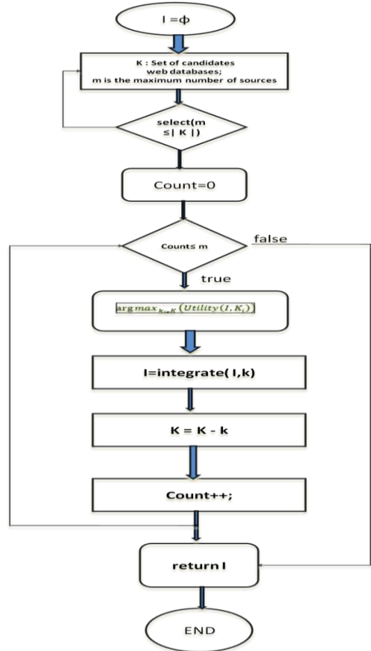
Figure 3: selection and Integration approach
