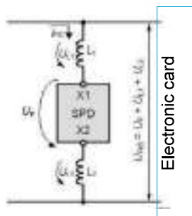
Connection of a Parallel SPD
