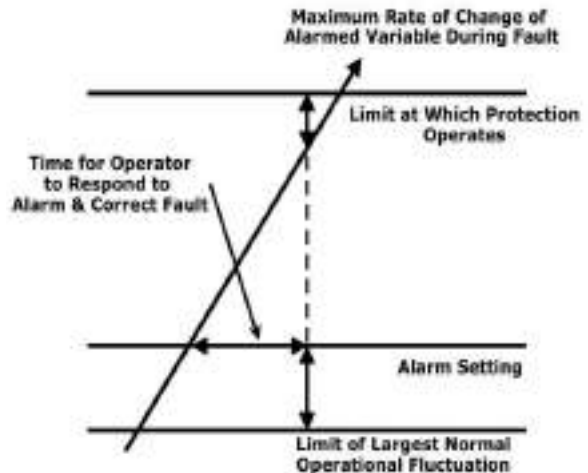
Alarm Settings Must Give Operators Appropriate Time to Respond to Faults Source: EEMUA Publication 191
