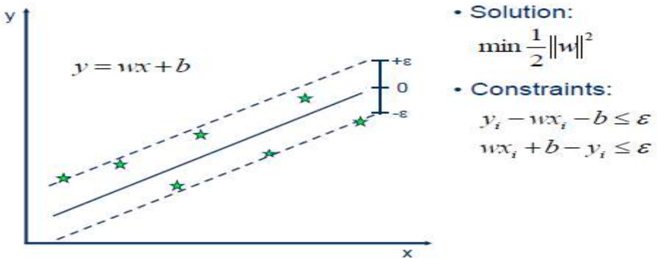
FIGURE-13:- SVM ALGORITHM
