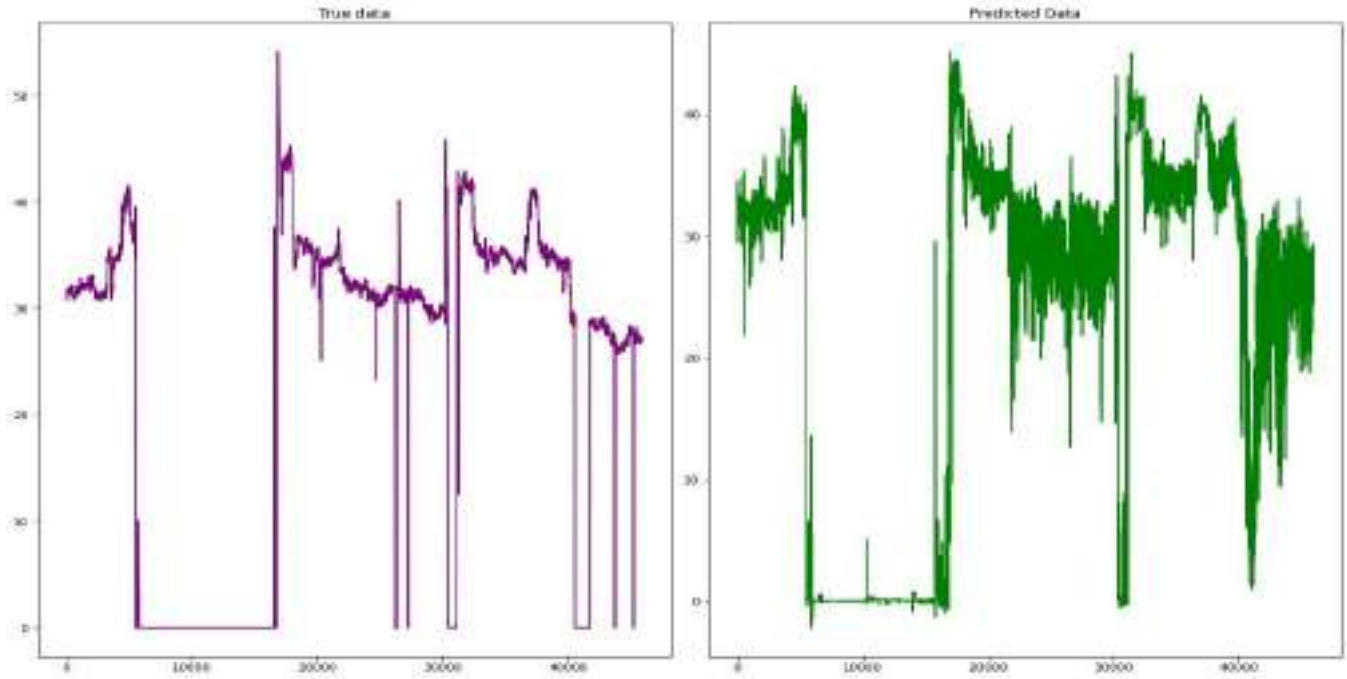
FIGURE-16:- C2H4 PREDICTION VS ACTUAL PLOTS FOR MODEL-1
