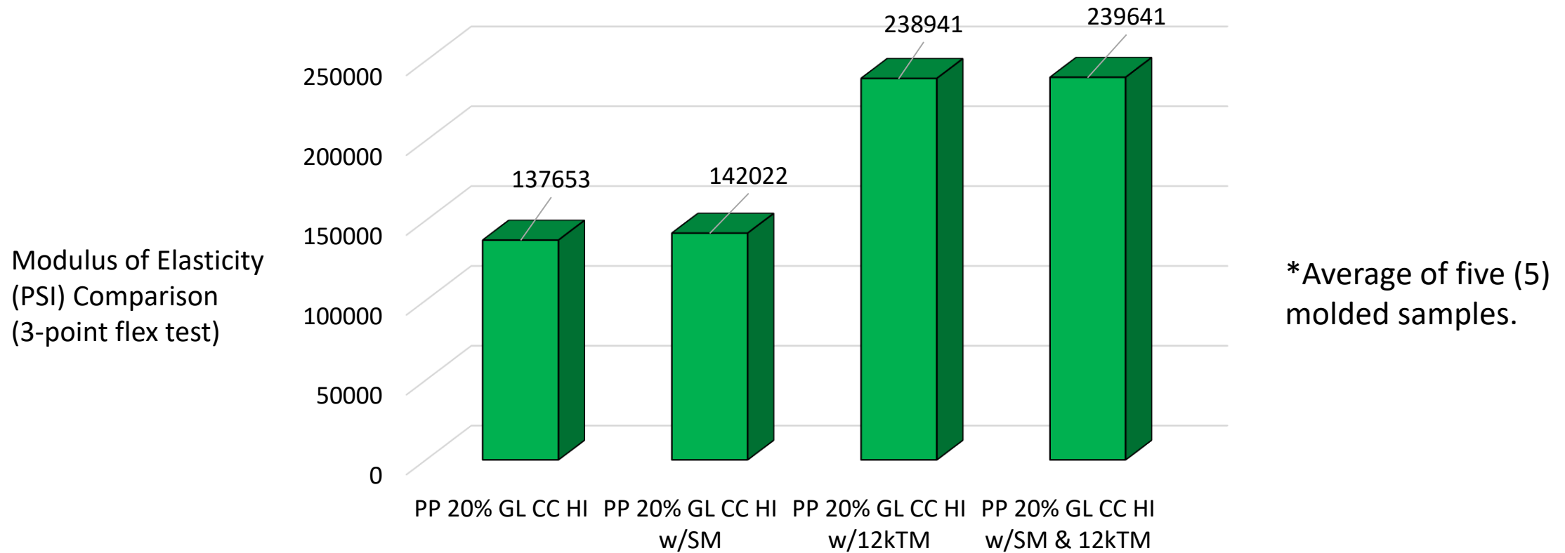
Injection Molded ICP 5" Panels Modulus of Elasticity 3-Point Testing (Ribs Down)
