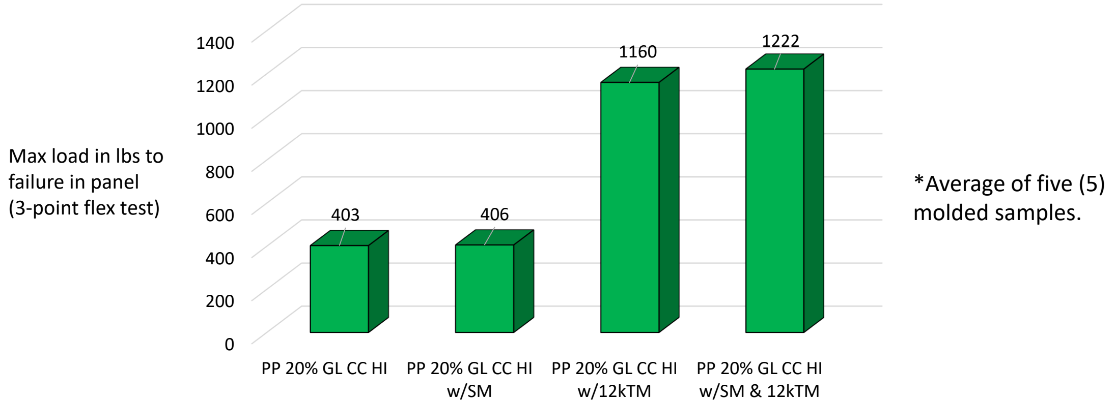
Injection Molded ICP 5" Panels Overall Strength 3-Point Flex Testing (Ribs Down)
