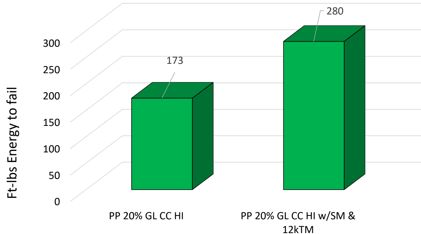
Injection Molded ICP 5" Test Panels Impact Data – Pendulum Tester
