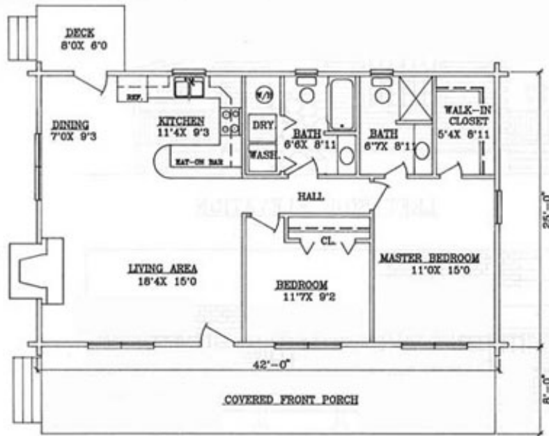
FLOOR PLAN
