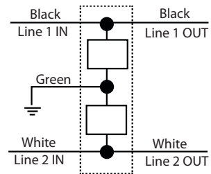
Wiring Diagram
