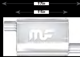
11" OFFSET/OFFSET
