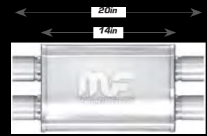
14" DUAL/DUAL
