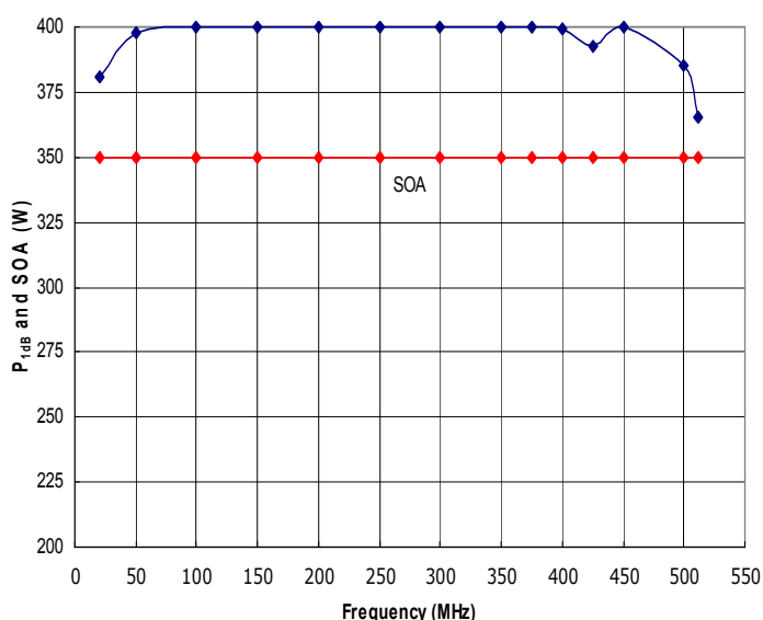
Figure 4: RFM20-512-350-HSD Typical P_{1dB} and Safe Operating Area (SOA). The amplifier is capable of delivering more power than it is safe to generate. Do not exceed the SOA shown above without first contacting RFMPT to discuss your application.
