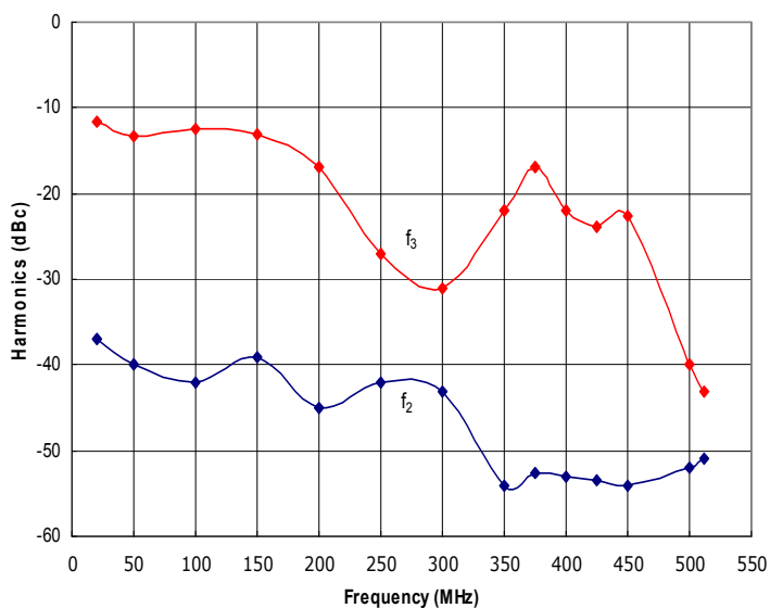
Figure 3: RFM20-512-350-HSD Typical f_2 and f_3 @ P_{out} = 350W .
