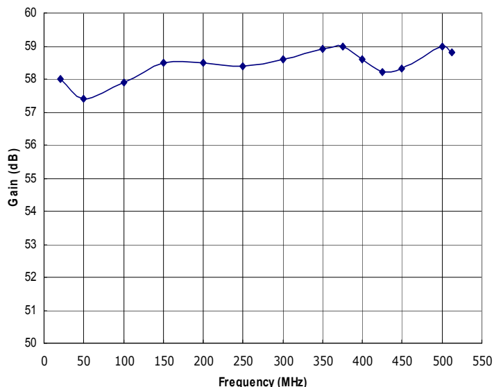
Figure 1: RFM20-512-350-HSD Typical Gain @ P_{out} = 350W .
