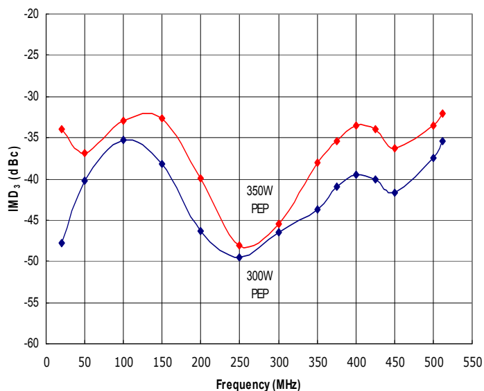
Figure 2: RFM20-512-350-HSD Typical IMD_3 @ 350W and 300W PEP, \Delta f = 100kHz .
