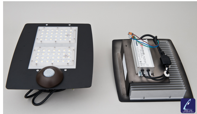
Cool-lite Retrofit Kit for Gullwing G13 Series
