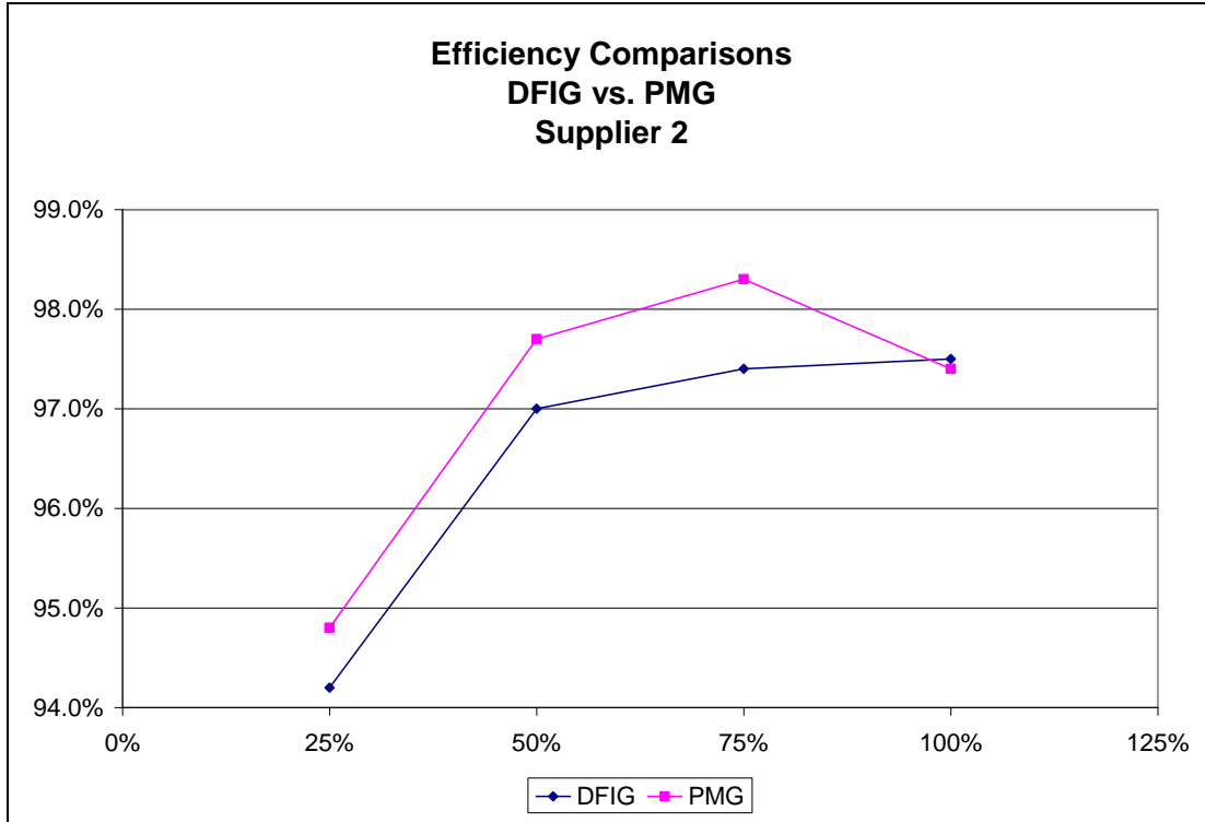
Figure 7: DFIG vs. PMG Efficiency Supplier 2
