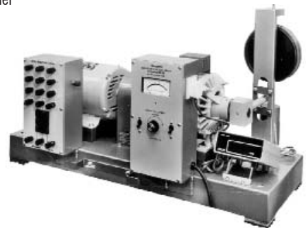
IM-300 Induction Motor coupled to MPB-300 Magnetic Particle Brake
