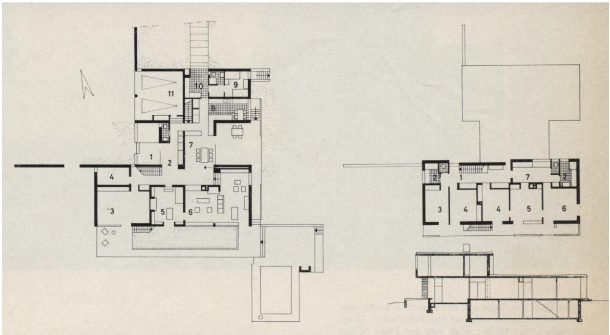
Floor Plans
