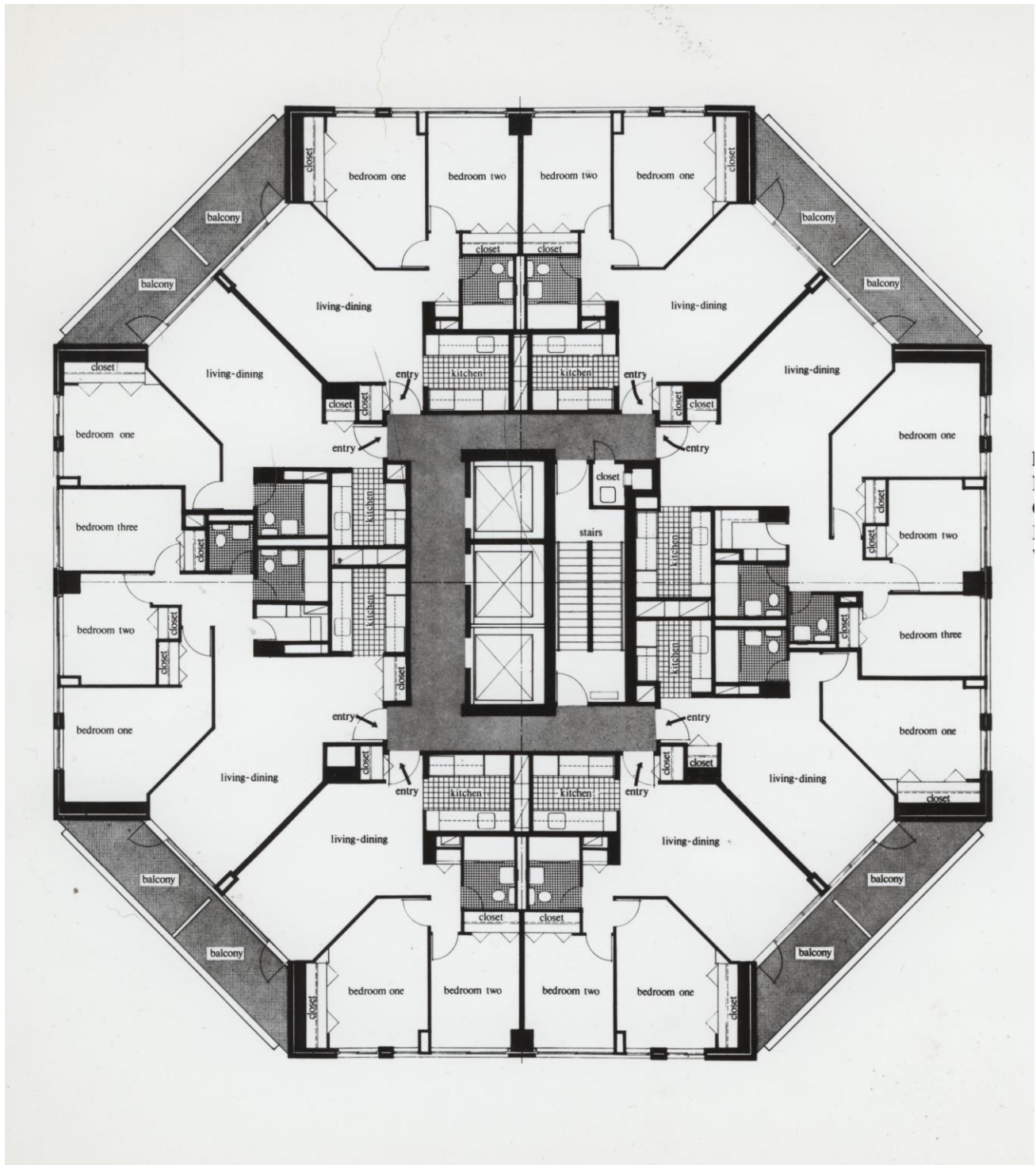
Schomburg Plaza Apartments, Typical Floor Plan, New York City
